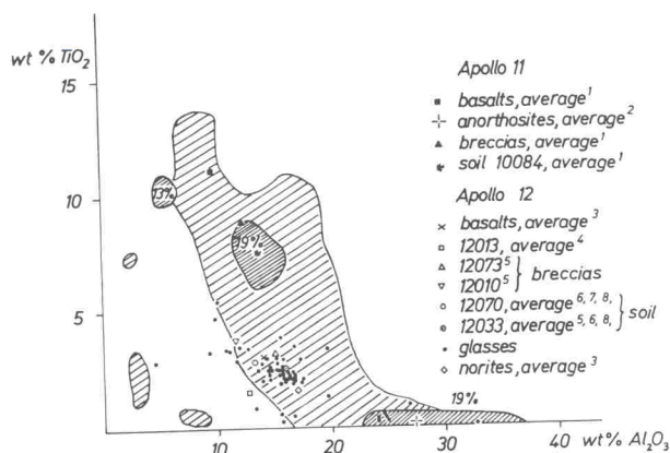
Fig. 5. TiO 2 versus Al 2 O 3 contents of glasses, igneous rocks, breccias and soil from Apollo 11 and Apollo 12. Glass analyses of this work (Apollo 12) are represented by dots. All hatched areas comprise 222 data points of Apollo 11 glass analyses taken from LEVINSON, Vols. 1 and 2 (1970). The narrow-hatched areas comprise the indicated percentages of all data points. References for all other data are designated by superior numerals and listed in caption of Fig. 8.
